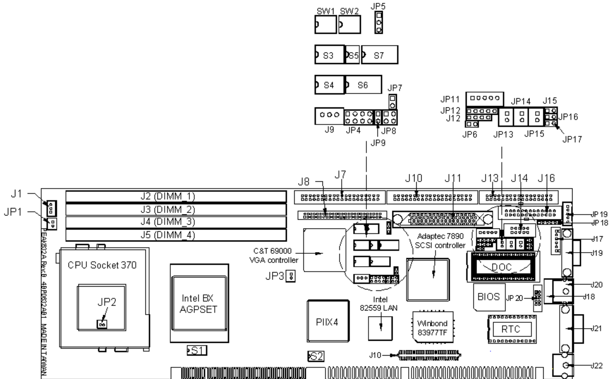
Figure 2-1 Switches and Connectors position
