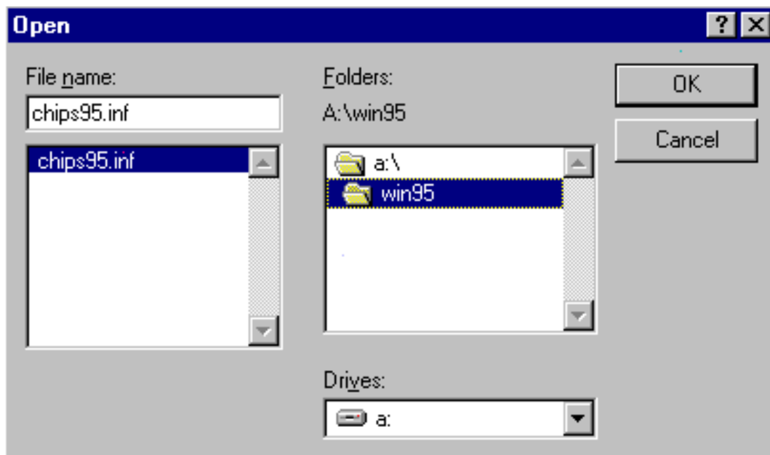
Figure 5-8: Selecting "chips98.inf"
